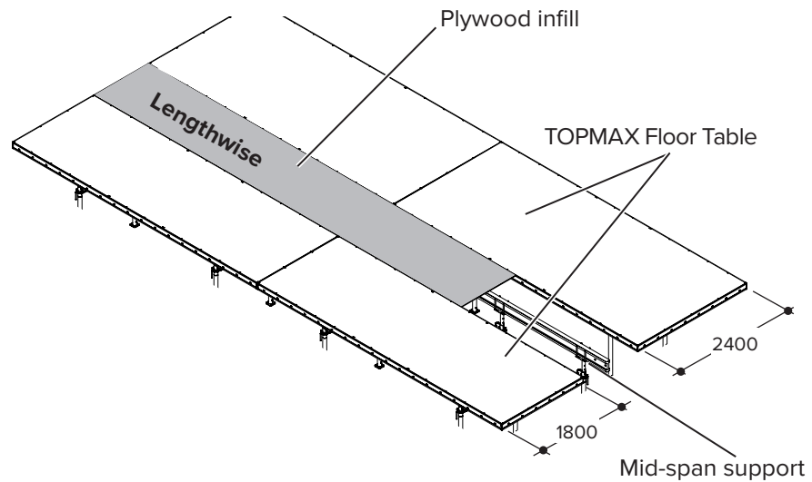
Infills lengthwise with mid-span support (table size 2.4 x 5.4)
