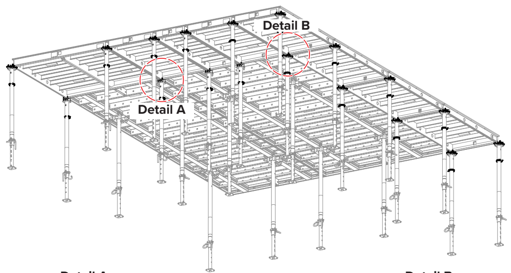
Detail A TOPMAX to TOPEC
